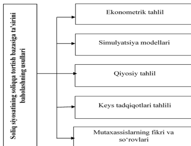
1-rasm. Soliq siyosatining soliqqa tortish bazasiga ta'sirini baholash metodlari 24
